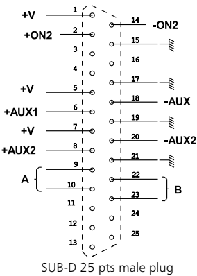
SUB-D 25 pts male plug
